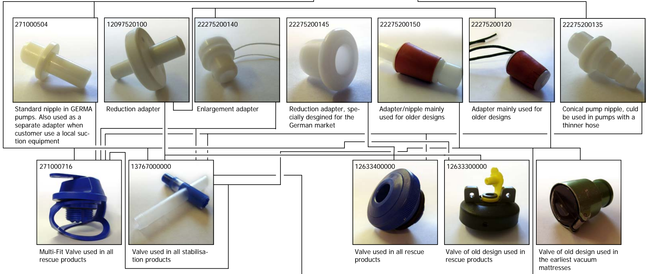
Pump or local suction equipment could together with adapters be used in vacuum products
